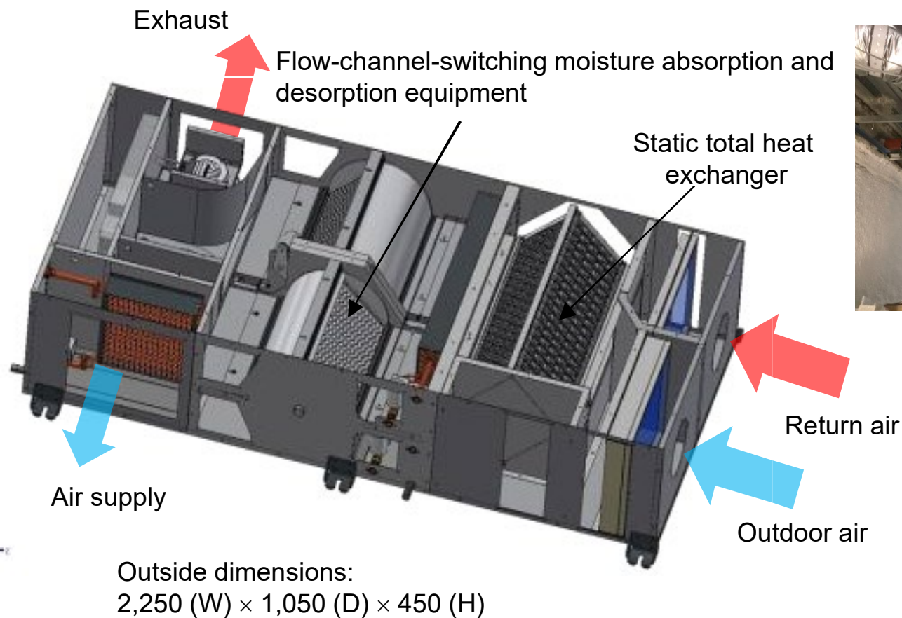
Internal structure of outside air handling unit for desiccant
