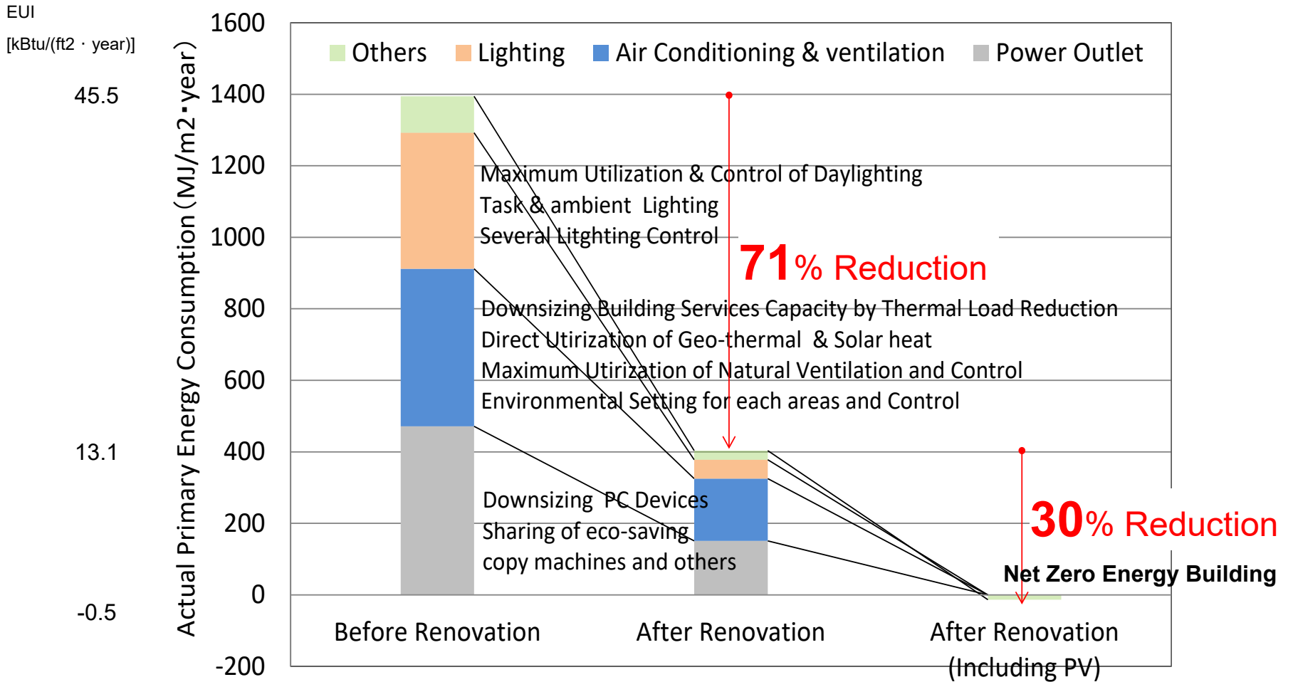
Comparison of primary energy consumption before and after renovation
